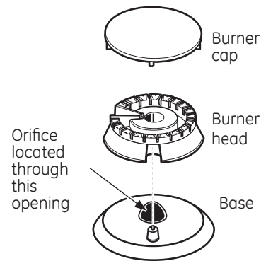
Burner construction
