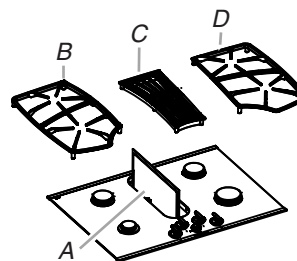
A. Grease filter B. Left side grate C. Center grate D. Right side grate
