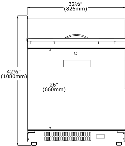
Front (UCSP132-SS11A)
